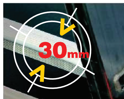
Piolo in alluminio estruso mm 30x30 antisdrucciolo , con angoli arrotondati 30x30 mm extruded aluminum anti-slip rung with rounded corners
